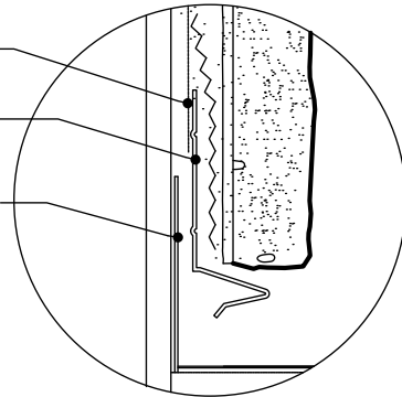
DETALLE 25.3
